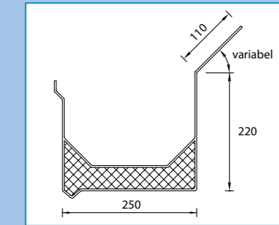
B-goot
