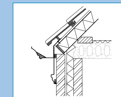
Smetplank Classic
