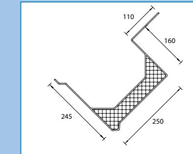
B-special
